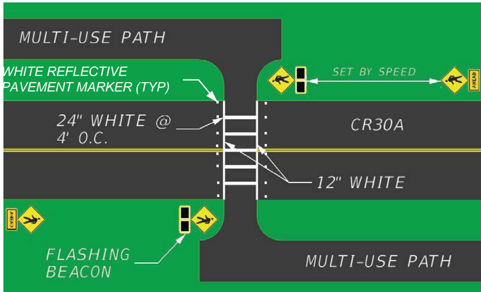
Figure 13. Recommended Trail Crossing Layout
