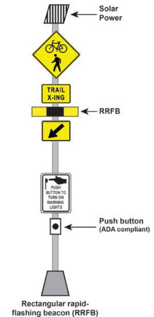
Figure 14. Example of RRFB
