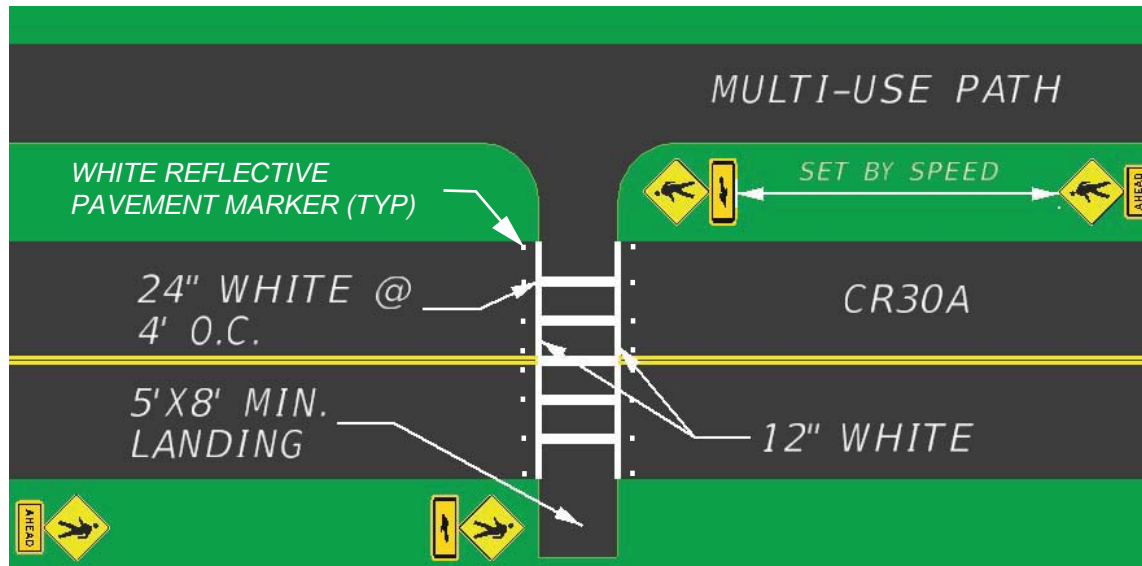
Figure 12. Recommended Minimum Crosswalk Layout
